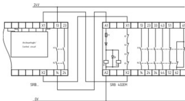
Wiring example
